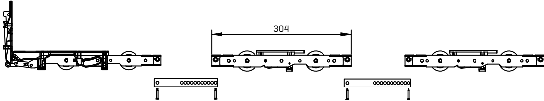
Assembly with 1 additional pulley [300 kg]
